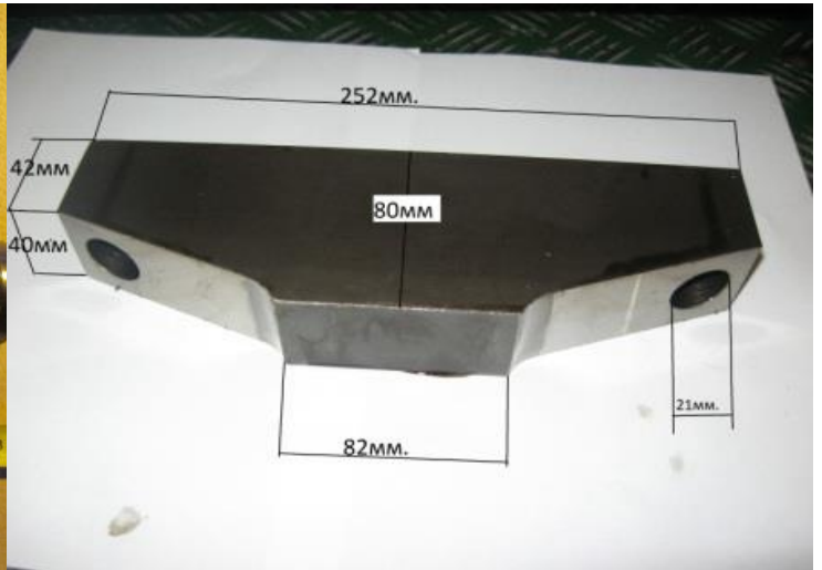
Thrust pad
